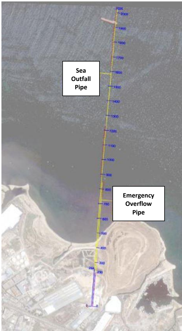
Figure 5-7: Sea Outfall Component
