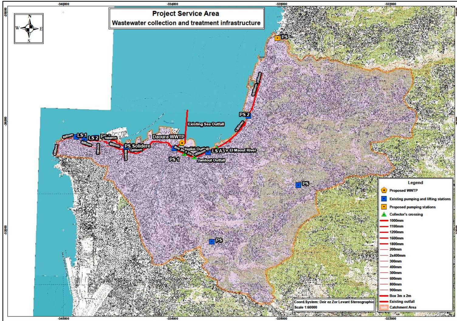
Figure 5-8: Project Service Area including Wastewater Collection and Treatment Infrastructure
